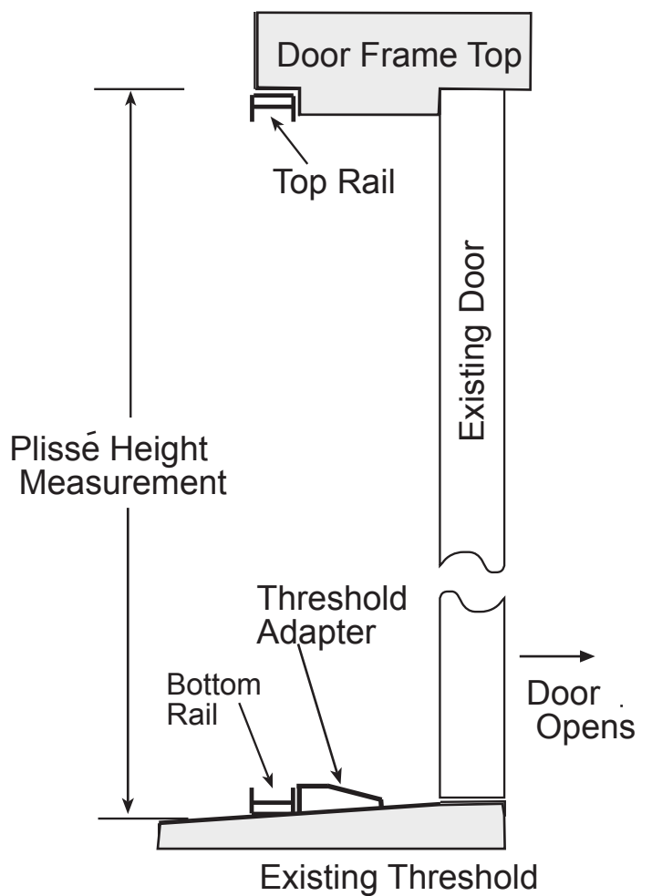
Typical Installation With Threshold Adapter
